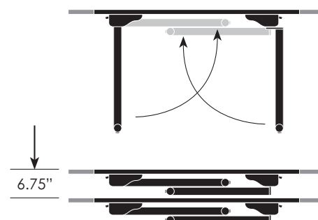
Short Folding
