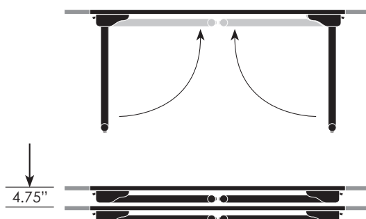
Standard Folding
