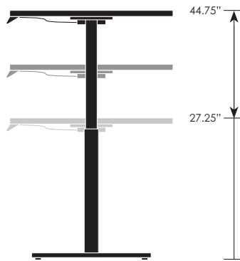
Electric T-bases
